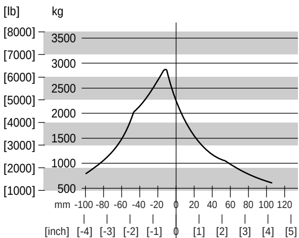
Standard Motor Straight Shaft
