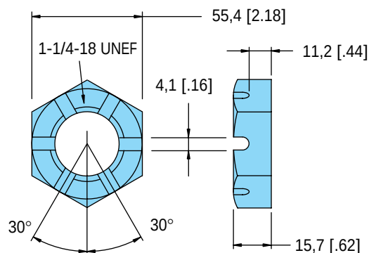
Slotted Hexagon Nut
